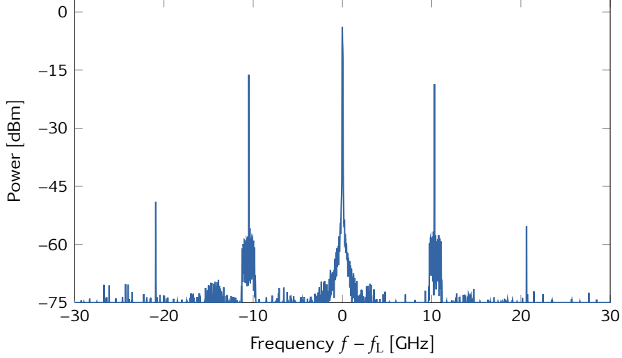
Figure 6: Optical spectrum of the signal at the through-port of the resonator. The central frequency f_L = 193\,276.6\text{GHz} is the optical frequency of the input laser. The sidemodes created by the MZ intensity modulator driven by the microwave oscillation are clearly visible on each side of the input frequency. The microwave noise from the amplifier is visible as a plateau on each side-mode, on top of which the oscillation at the FSR frequency stands. It is apparent on this figure that the amplitudes of the sidemodes decreases very rapidly, so that only few of them are necessary to describe the behavior of the oscillator in the numerical simulations.
