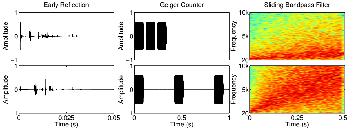
Figure 2: Representation of the sound resulting from the application of the three effect metaphors for two distances: top = 0.6 m, bottom = 1.5 m; (Left) Impulse response of the Early Reflection effect metaphor. (Center) Geiger Counter effect metaphor applied to a 10 ms burst. (Right) Spectrogram of the sounds resulting from the Sliding Bandpass Filter effect metaphor applied to a 0.5 sec burst.
