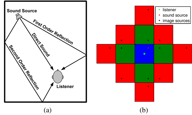
Figure 1: (a) Sound path in a room. (b) 2D schematization of the image-sources method. The simulated room is in blue, first order reflections are located in green areas and second order reflections are located in red areas. The listener is a green ●, the source a red ●.
