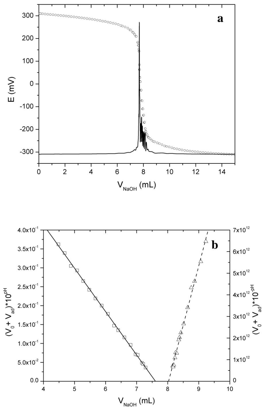
FIGURE 1. (a) Titration of \text{HNO}_3 with \text{NaOH} after contact with BP- \text{H}_2\text{O} (open circles) and the corresponding derivate (continuous line). (b) Gran representation for the titration showed in (a). Acid regression (squares) and basic regression (triangles) with the corresponding linear fits, \psi and \psi' .
