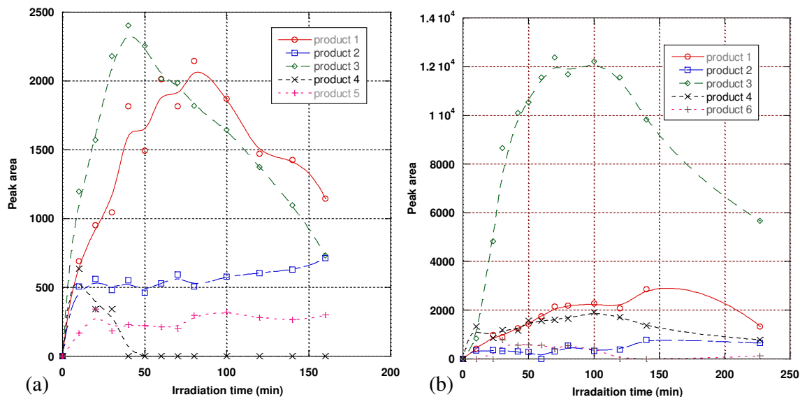
Fig. 4 – Monitoring of BPA intermediates formed when using P25 (a) and ECT-1023t (b) under UV-visible irradiation (200 nm–30 μm).
