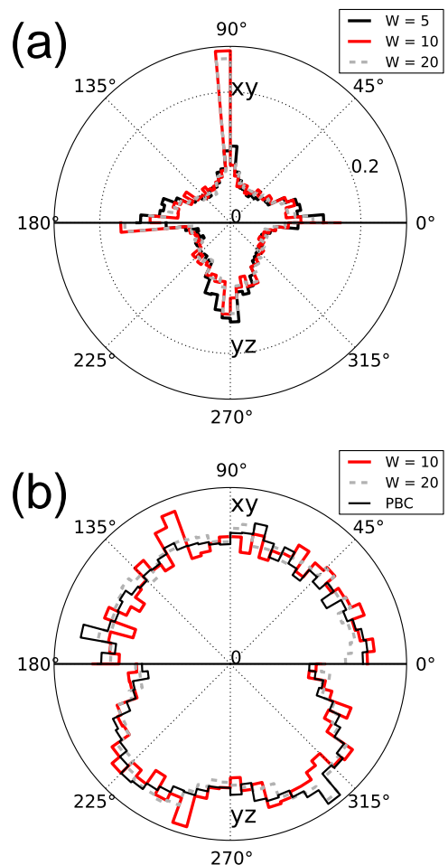
FIG. 12. (Color online) Contact normal orientation distributions for MPP inside the boundary layers (a), and inside the bulk region (b). The upper half of each chart (e.g. from 0 to 180^\circ ) corresponds to the xy plane, while the lower half corresponds to the yz plane. Several gap widths are considered.
