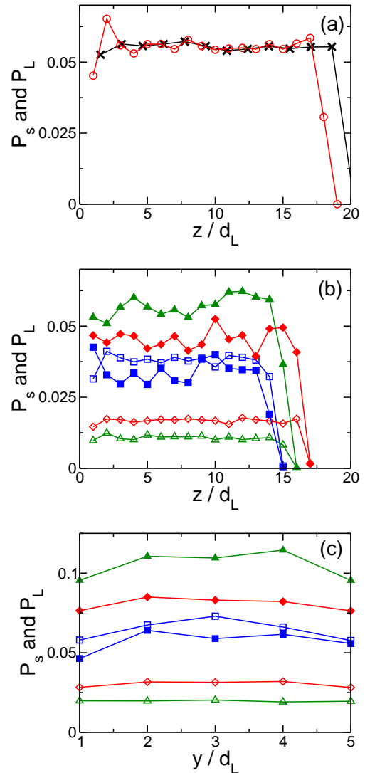
FIG. 5. (Color online) (a) Homogeneity of MSP ( \circ ) and MPP ( \times ) along the z axis, expressed as the ratio of the number of grains to the total number of grains in d_L -thick layers. (b) Homogeneity of BSP along the z axis, expressed as the ratio of the number of large (empty symbols) and small (solid symbols) grains to the total number of grains in d_L -thick layers for x_s = 10\% ( \square ), x_s = 25\% ( \diamond ) and x_s = 40\% ( \triangle ). (c) Homogeneity of BSP along the y axis, same calculation method and same key. For (a), (b), and (c), the gap between sidewalls is W = 5d_L and the data have been averaged over three simulations.
