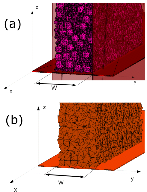
FIG. 2. (Color online) Typical 3D snapshots of packings made of polysized spheres (a) and pinacoids (b). The confinement is characterized by the gap W between sidewalls. The direction of gravity is -z .
