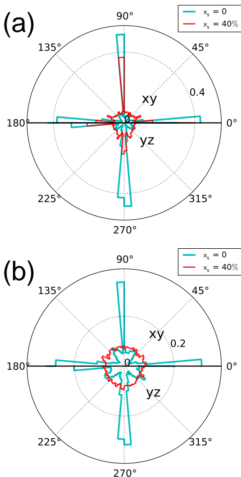
FIG. 11. (Color online) Contact normal orientation distributions for MSP ( x_S = 0 ) and BSP ( x_S = 40\% ) inside the boundary layers/closer than 1.5d_L to a sidewall (a) and inside the bulk region (b). The upper half of each chart (e.g., from 0 to 180^\circ ) corresponds to the xy plane, while the lower half corresponds to the yz plane. The gap width is W = 5d_L and the bulk region coincides with particles located at least 1.5d_L away from the sidewalls.
