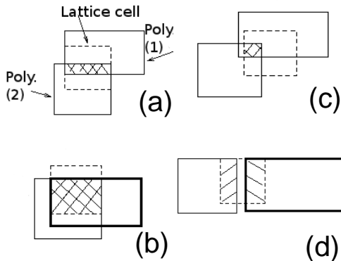
FIG. 4. 2D simplified representation of the four intersection situations between two pinacoids and a lattice cell: (a) solid volume \geq cell volume and partial interpenetration in the cell; (b) solid volume \geq cell volume and total interpenetration in the cell; (c) solid volume < cell volume and interpenetration (partial as represented or total); and (d) solid volume < cell volume and no interpenetration.
