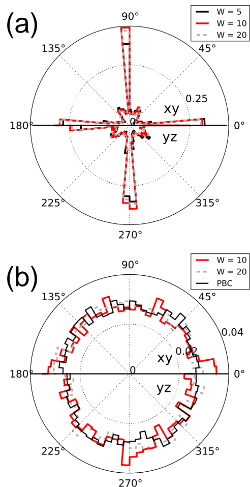
FIG. 10. (Color online) Contact normal orientation distributions for MSP inside the boundary layers (a) and inside the bulk region (b). The upper half of each chart (e.g., from 0 to 180°) corresponds to the xy plane, while the lower half corresponds to the yz plane. Several gap widths are considered.
