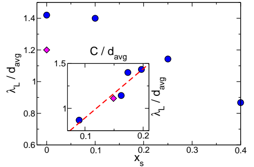
FIG. 8. (Color online) Characteristic length of confinement effect \lambda_L versus fraction of small grains x_s for MSP and BSP (circle) as well as for MPP (diamond) with W = 10d . That length is defined in Eq. 8. The effect of confinement is found to decrease with increasing grain polydispersity or grain angularity. The inset reports the same length versus that of the fit parameter in Eq. (1): C = 2h(\phi_{bulk} - \Phi_{BL}) . The dashed line corresponds to a linear fit.
