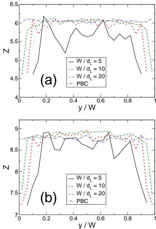
FIG. 15. (Color online) Coordination number profiles (along y ) for MSP (a) and for MPP (b) for several gap width. These profiles evidence a constant central zone and two drop zones in contact with the sidewalls.
