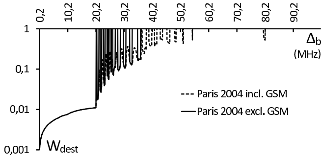
Figure 15: probability of destruction of an APC by a TCR as a function of the frequency shift \Delta_b between consecutive quantum states in well (b), in Paris in 2004 including and excluding GSM.
