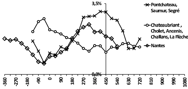
Figure 20: ratios of yearly mortality in the 35-44 years age range over total yearly mortality, as a function of time (in days). The curve of Nantes has a starting date on 4th june 2010 approximately corresponding to the increase in authorized power in the corresponding emitter of Haute-Goulaine. The other places have a starting date on 5th February 2010 corresponding to authorization of the emitters of Pontchateau, Saumur, segré.
