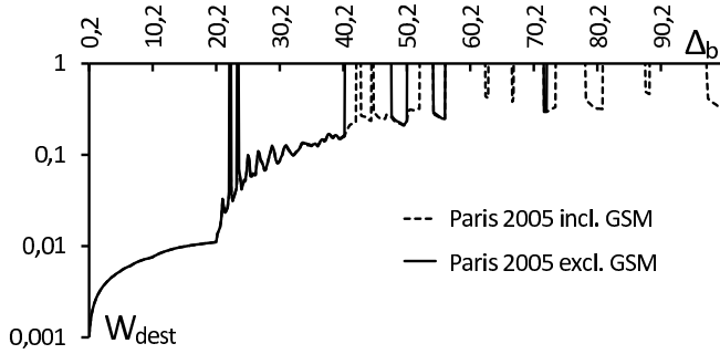
Figure 16: probability of destruction of an APC by a TCR as a function of the frequency shift \Delta_b between consecutive quantum states in well (b), in Paris in 2005 including and excluding GSM.
