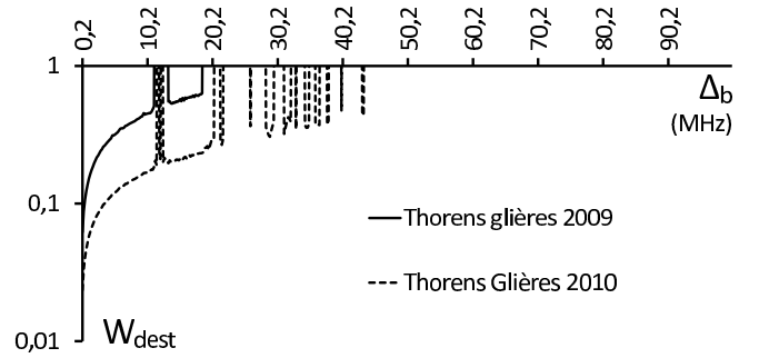
Figure 10: probability of destruction of an APC by a TCR as a function of the frequency shift \Delta_b between consecutive quantum states in well (b), in Thorens-Glieres prior to (2009) and after (2010) start-up of DVB
