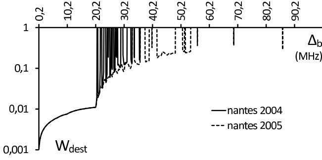
Figure 8: probability of destruction of an APC by a TCR as a function of the frequency shift \Delta_b between consecutive quantum states in well (b), in Nantes prior to (2004) and after (2005) start-up of DVB
