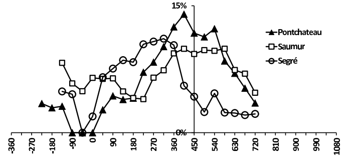
Figure 17: ratios of yearly mortality in the 35-54 years age range over total yearly mortality, as a function of time (in days), for places having received DVB emitters authorized by the ANFR (Agence Nationale des Fréquences) on 5th February 2010 and having discontinued analog TV emission on 18th May 2010 in the region "Pays de Loire", with a starting date on 5th February 2010.
