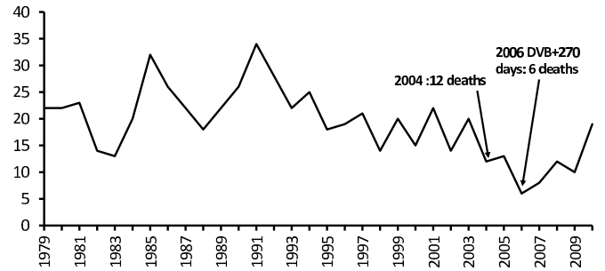
Figure 22: yearly number of deaths in the 35-44 years age range for men only in Paris corresponding to neoplasms of the lung, trachea and bronchial tubes
