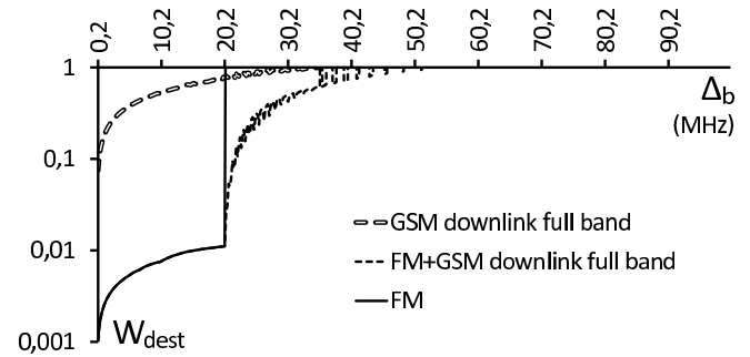
Figure 14: probability of destruction of an APC by a TCR as a function of the frequency shift \Delta_b between consecutive quantum states in well (b), for various combinations of FM radio and GSM downlink. Average FM spectral power is equal to peak GSM spectral power
