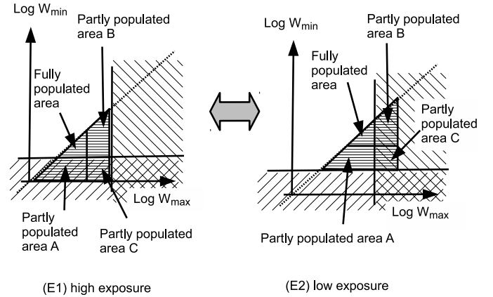
Figure 13: selection of T cells by the thymus in an alternating high/low exposure situation.
