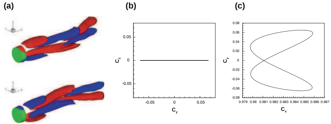
Fig. 5 Periodic mode with reflectional symmetry and zero mean lift (or “Zig-Zag” mode) for Re = 216 . a Iso-levels of the streamwise vorticity in the plane located at x = 0.5 , b C_y - C_z diagram, c C_x - C_L diagram
