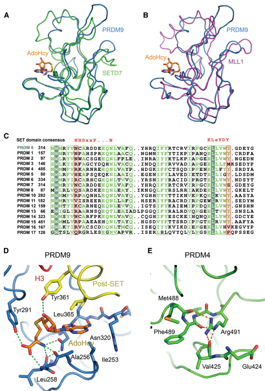
Figure 2. AdoHcy Binding by PRDM Proteins
