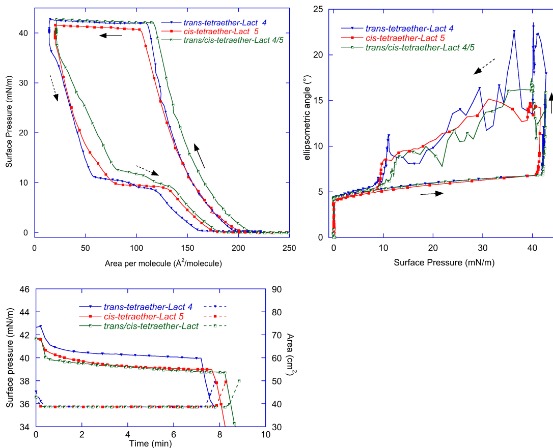
Fig. 5 Compression/decompression isotherms of trans -tetraether-Lact 4 , cis -tetraether-Lact 5 and trans/cis -tetraether 4/5 and Relaxation of about 7 min at constant area at collapse (30% of points shown, arrows correspond to compression (plain line) and expansion (dotted line)).
