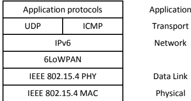
Figure 3. Basic structure of 6LoWPAN stack
