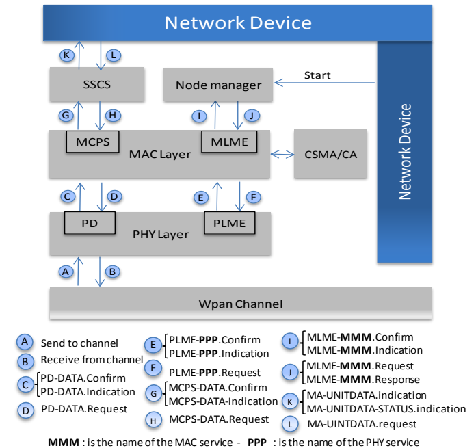
Figure 4. WPAN model architecture
