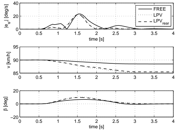
Fig. 8. Yaw rate error, speed and body slip angle: LPV (dotted), LPV with rear steer (dashed). Uncontrolled vehicle (black)
