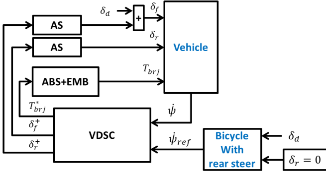
Fig. 1. Control architecture. AS are the active steering actuators and ABS+EMB are the wheel torque actuators (at the left/right rear wheels).
