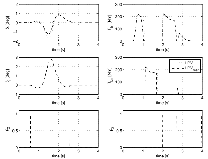
Fig. 9. Control inputs: LPV (dotted), LPV with rear steer (dashed).
