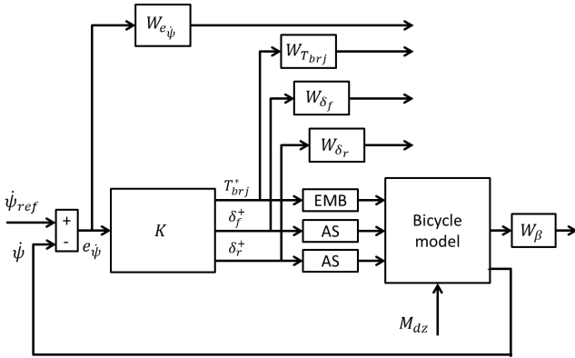
Fig. 2. Generalized plant used for synthesis.
