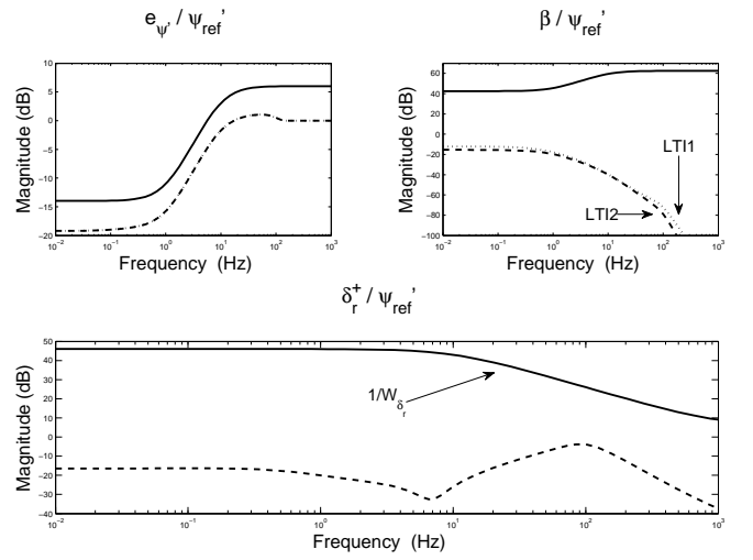
Fig. 3. LTI controller, frequency response: LTI1 (black dotted), LTI2 (black dashed). Weighting functions 1/W_{e_\psi}, 1/W_\beta, 1/W_{\delta_r^+} (black solid).
