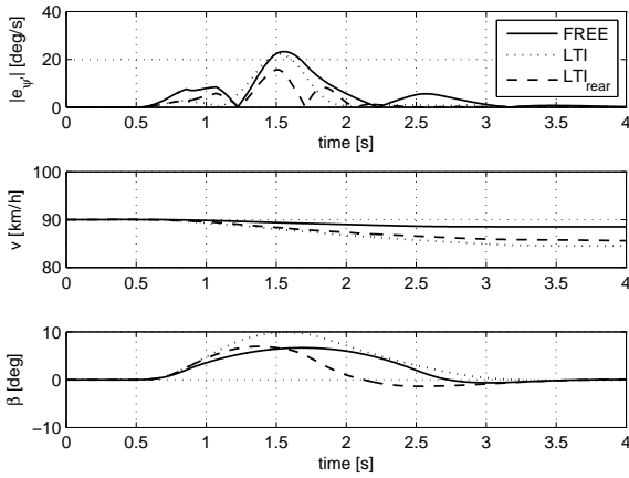
Fig. 6. Yaw rate error, speed and body slip angle: LTI (dotted), LTI with rear steer (dashed). Uncontrolled vehicle (black)
