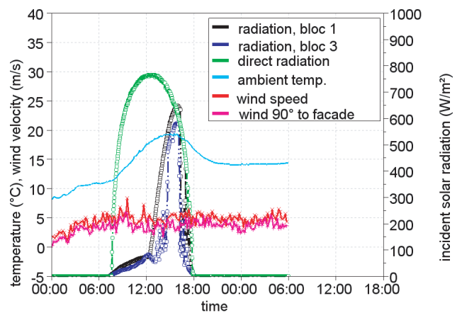
Figure 6: Radiation, temperature, and wind for one sunny day (above) and one windy day (below).
