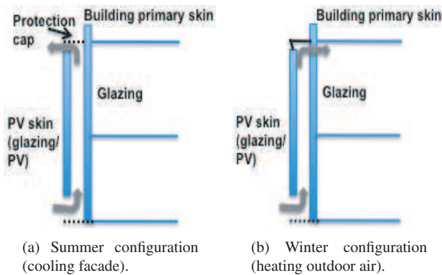
Figure 1: Operating principal of the double skin in addition to classical envelope function.
