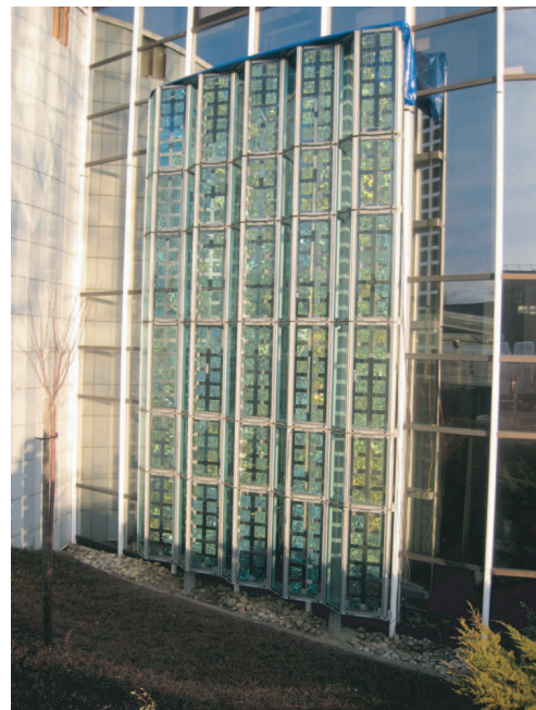
Figure 3: Double-skin prism facade.
