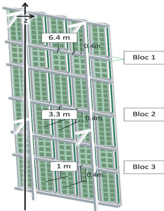
Figure 4: Spatial arrangement of “peignes” in the air gap.
