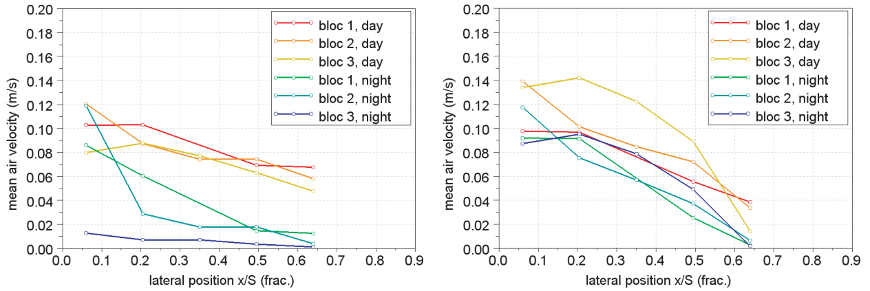
Figure 7: Mean velocity profile between the external and internal facades for a typical sunny day (left) and a typical sunny and windy day (right).
