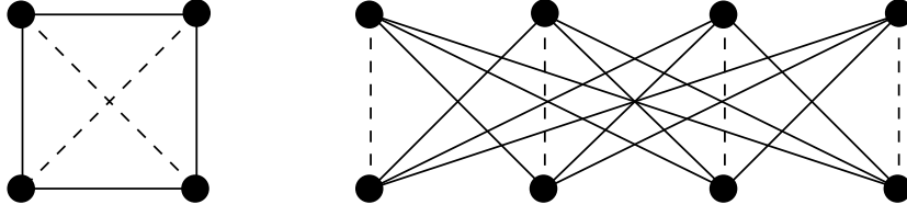
Fig. 1: Signed projective cubes of dimension 2 and 3
