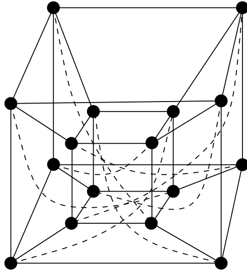
Fig. 2: Signed projective cube of dimension 4
