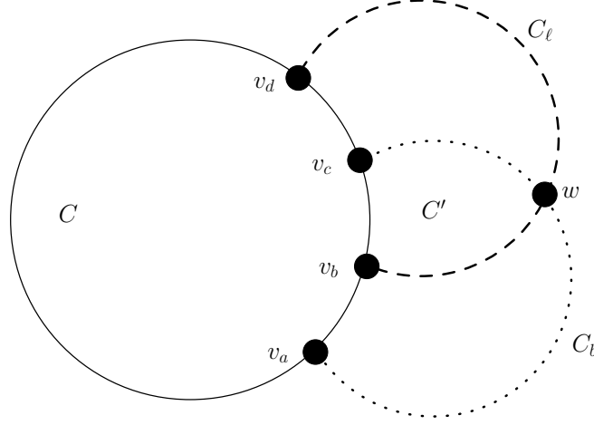
Fig. 3: Configuration for the proof of Lemma 3.1
