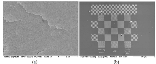
Fig. 6. (a) Gold on carbon sample (b) Microscale calibration rig.
