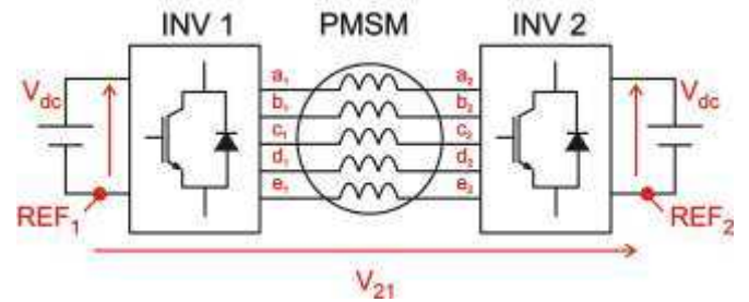
Fig. 1: Drive topology
