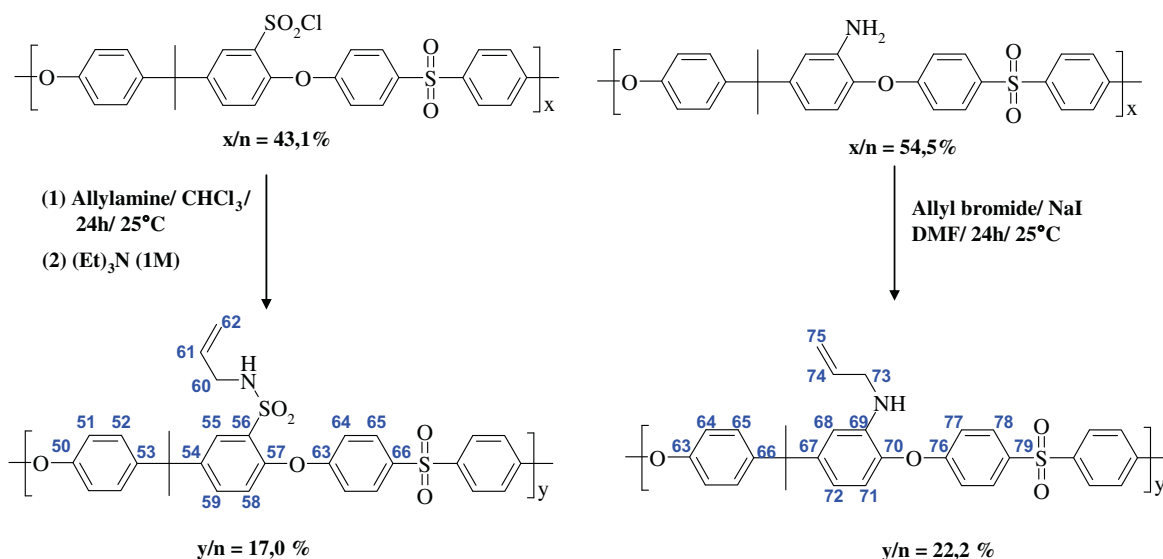
Scheme 2. Alkylation of aminated and sulfonated polysulfones.
