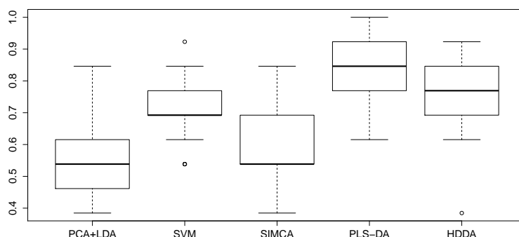
Figure 5: Boxplots of correct classification rates obtained by 25-fold double cross validation for PCA+LDA, SVM, SIMCA, PLS-DA and HDDA for the prostate data set.
