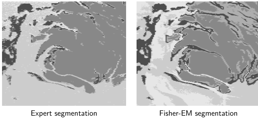
Figure 10: Segmentation of the hyperspectral image of the Martian surface using a physical model build by experts (left) and Fisher-EM (right).
