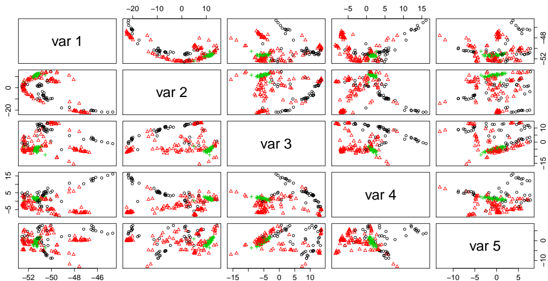
Figure 2: Scatter plot of the 3-class NIR data projected onto the 5 first principal axes.
