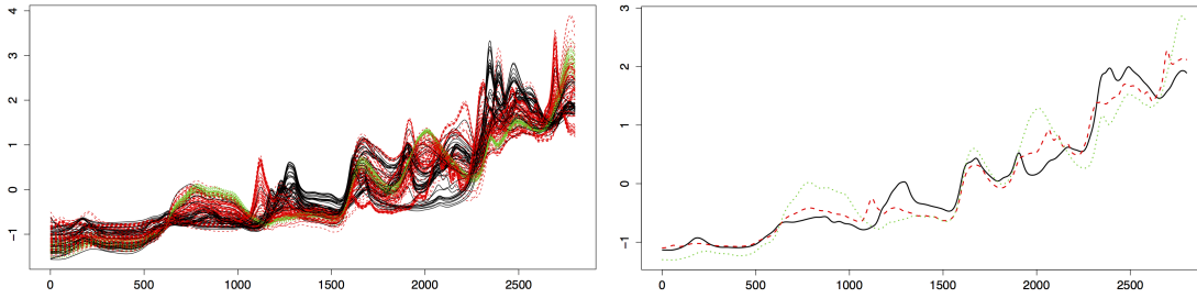
Figure 1: Spectra of the 3-class NIR data set (top) and mean of each class (bottom).
