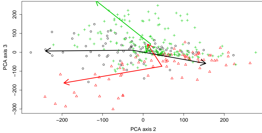
Figure 6: Projection of the estimated class-specific subspaces onto the principal components (PCA axes 2 and 3) for the prostate data set.
