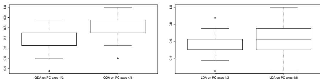
Figure 3: Boxplots of correct classification rates obtained by 25-fold cross validation for QDA (left) and LDA (right) on the PCA axes 1/2 and 4/8.
