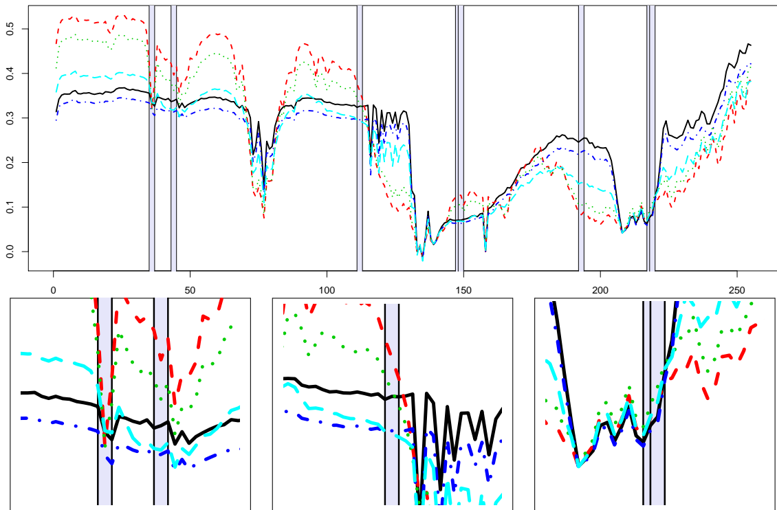
Figure 11: Mean spectra of the 5 groups formed by sparseFEM and selection of the discriminative wavelengths (indicated by gray rectangles). Some details are shown at the bottom to ease the visualization.
