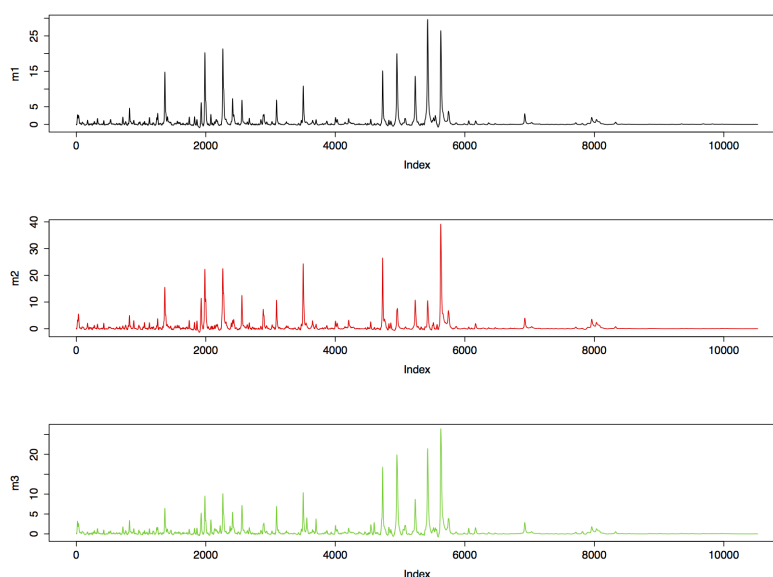
Figure 4: Mean spectra of the three classes for the prostate data set.
