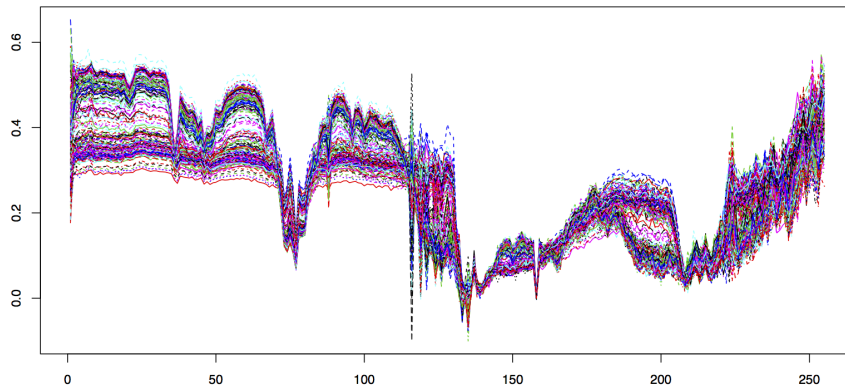
Figure 8: Some of the 38 400 measured spectra described on 256 wavelengths from 0.36 to 5.2 \mu\text{m} (see text for details).
