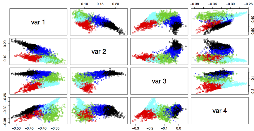
Figure 9: Projection of the clustered data on the estimated discriminative axes with Fisher-EM for the Mars data set.
