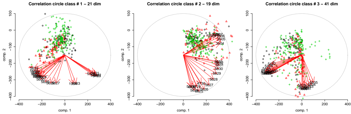
Figure 7: Correlation circles for the three classes of the prostate data set.
