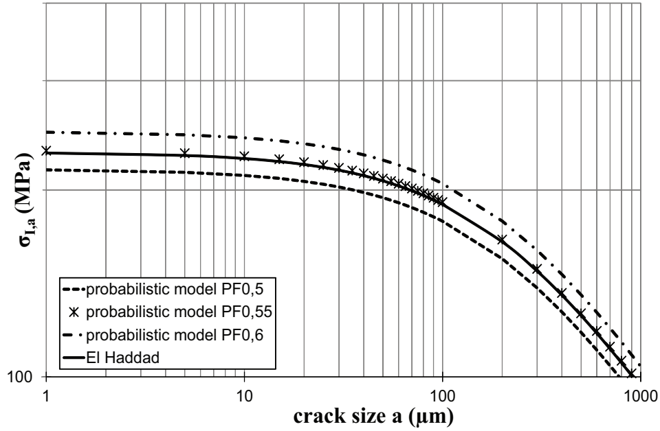
Fig. 5: Kitagawa-Takahashi diagram: comparison between the El Haddad approach and the proposed probabilistic model for uniaxial push-pull loads ( \Delta K_{th} = 11.9MPa.m^{1/2} , S_{-1} = 230MPa , m = 2.0 , \sigma'_{th01} = 260MPa , Y = 1.0 , \Delta K'_{th02} = 13.4MPa.m^{1/2} )
