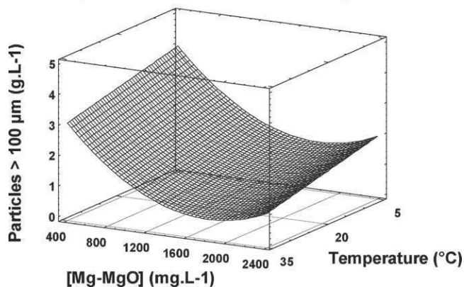
Fig. 9. [Mg-MgO] and temperature negatively influence concentration of particles bigger than 100 μm, the grid represents the surface response of the statistical model.
