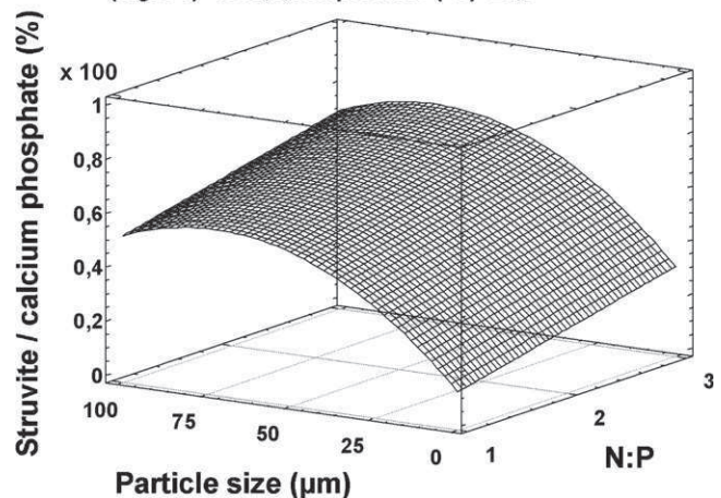
Fig. 10. Particle size and N:P molar ratio positively influence the proportion of struvite versus calcium phosphate in dried solid, the grid represents the surface response of the statistical model.
