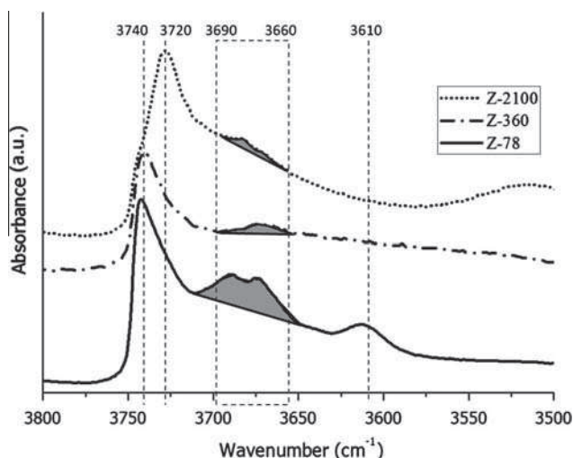
Fig. 1. IR spectra of hydroxyl region of ZSM-5 zeolites: Z-78, Z-360, Z-2100. Activation conditions: 12 h in air flow ( 1 \text{ cm}^3 \text{ s}^{-1} ) at 500 ^{\circ}\text{C} and then using vacuum ( 1.33 \times 10^{-4} \text{ Pa} ) at 400 ^{\circ}\text{C} for 1 h. NB: The curves are offset for a better readability.
