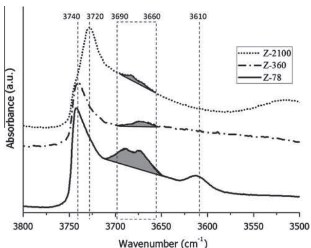
Fig. 1. IR spectra of hydroxyl region of ZSM-5 zeolites: Z-78, Z-360, Z-2100. Activation conditions: 12 h in air flow ( 1 \text{ cm}^3 \text{ s}^{-1} ) at 500 ^{\circ}\text{C} and then using vacuum ( 1.33 \times 10^{-4} \text{ Pa} ) at 400 ^{\circ}\text{C} for 1 h. NB: The curves are offset for a better readability.
