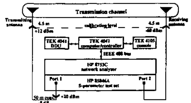
Fig. 1. Measurement system
