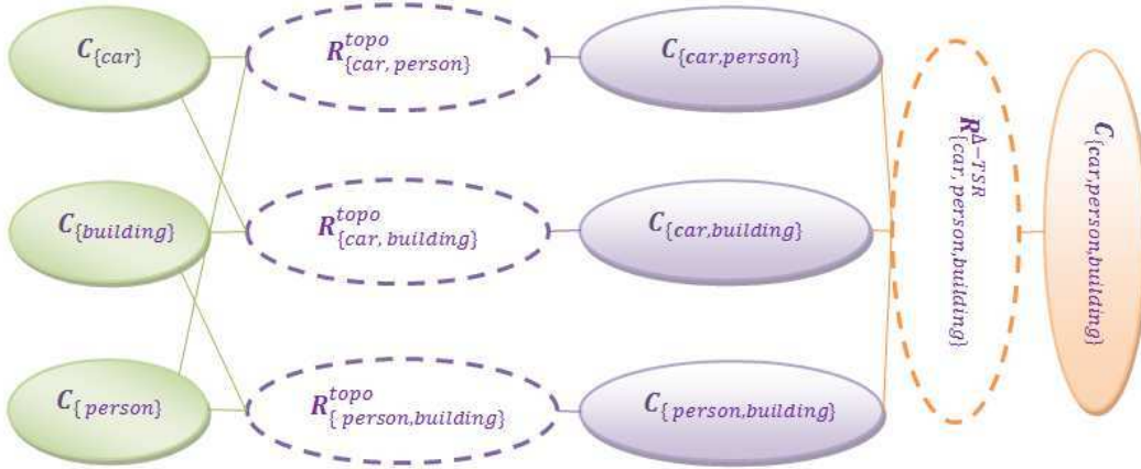
(c) Inferences at step 2 : inferences of the R nodes
