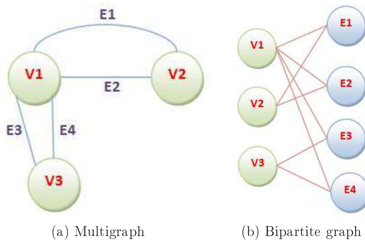
FIGURE 4 – An example of multigraph and its bipartite representation.
