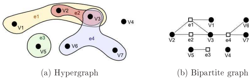
FIGURE 3 – An example of hypergraph and its bipartite representation.
