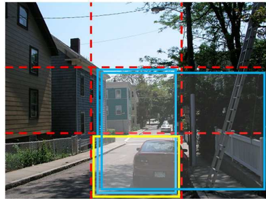
(b) Detection of "car"
