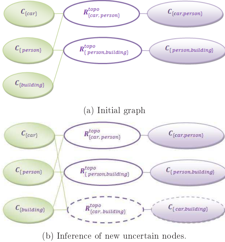
FIGURE 14 – Example of automatic inferences in the graph.
