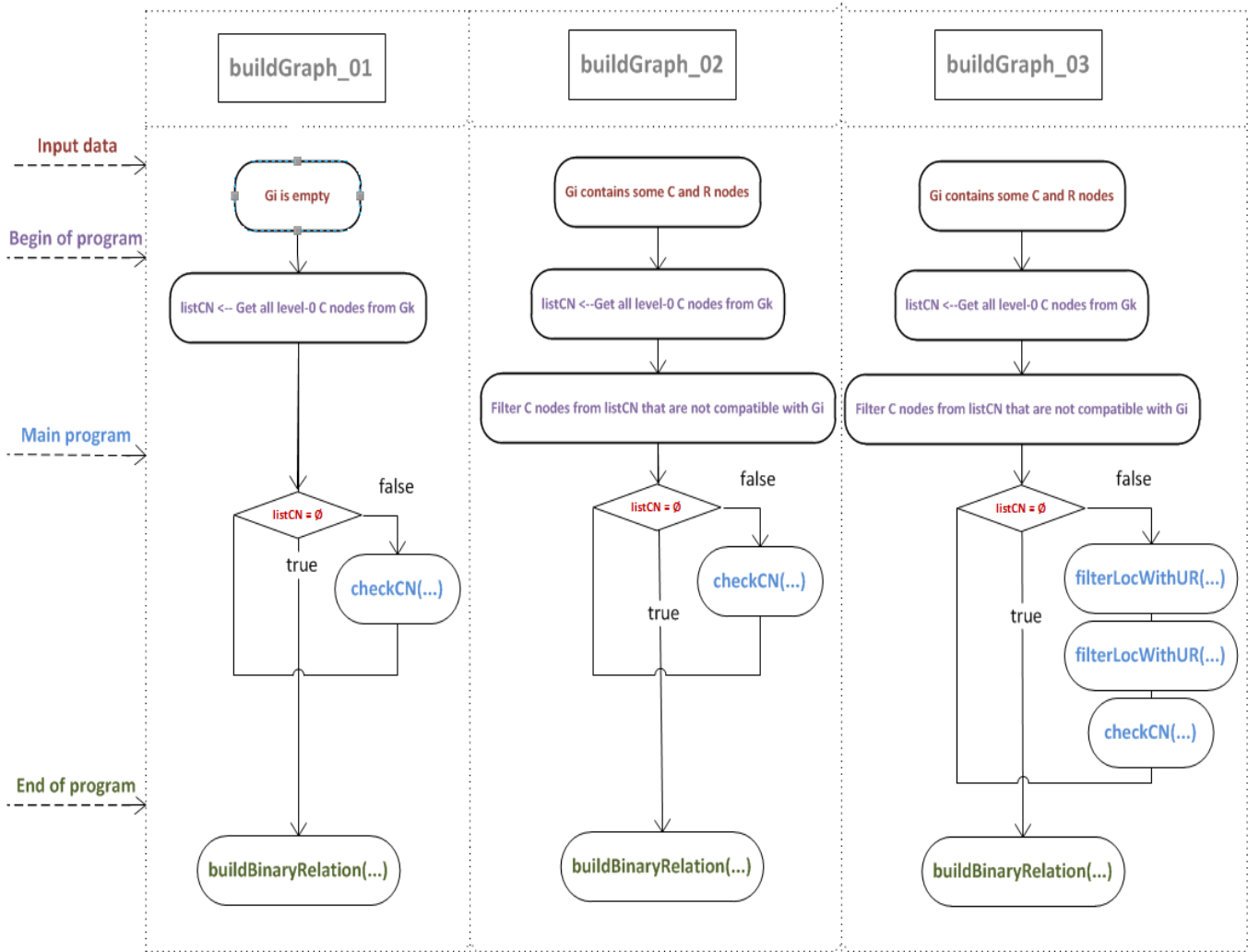
FIGURE 19 – An overview of the three graph building algorithms for a given image.
