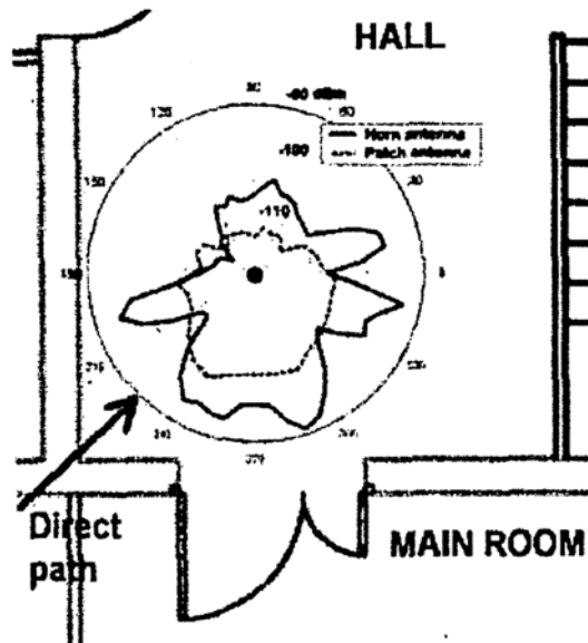
Figure 5. Received power for RX07 in the C.L.E.
