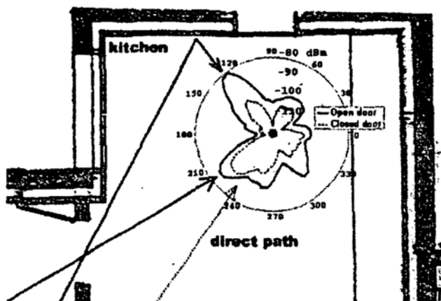
Figure 4. Received power for RX05 in the House.
