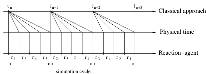
Fig. 1. Classical and reaction-agent points of view for reactions scheduling. Case of 4 reaction-agents r_i, 1 \leq i \leq 4 .
