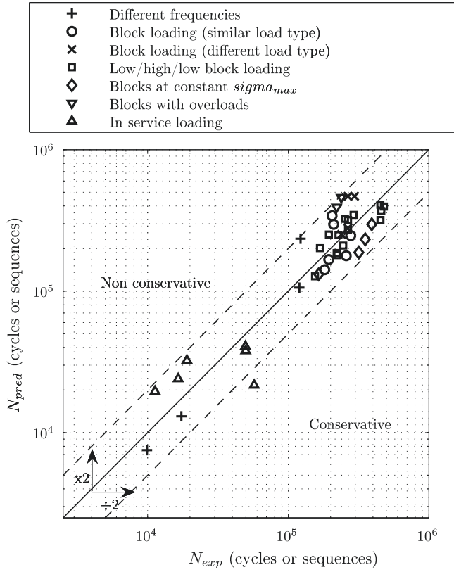
Fig. 10. Experimental and simulated fatigue lives (for in service loadings fatigue life is expressed in number of load sequences) for different loading cases on EN-GJS800-2 smooth specimens.
