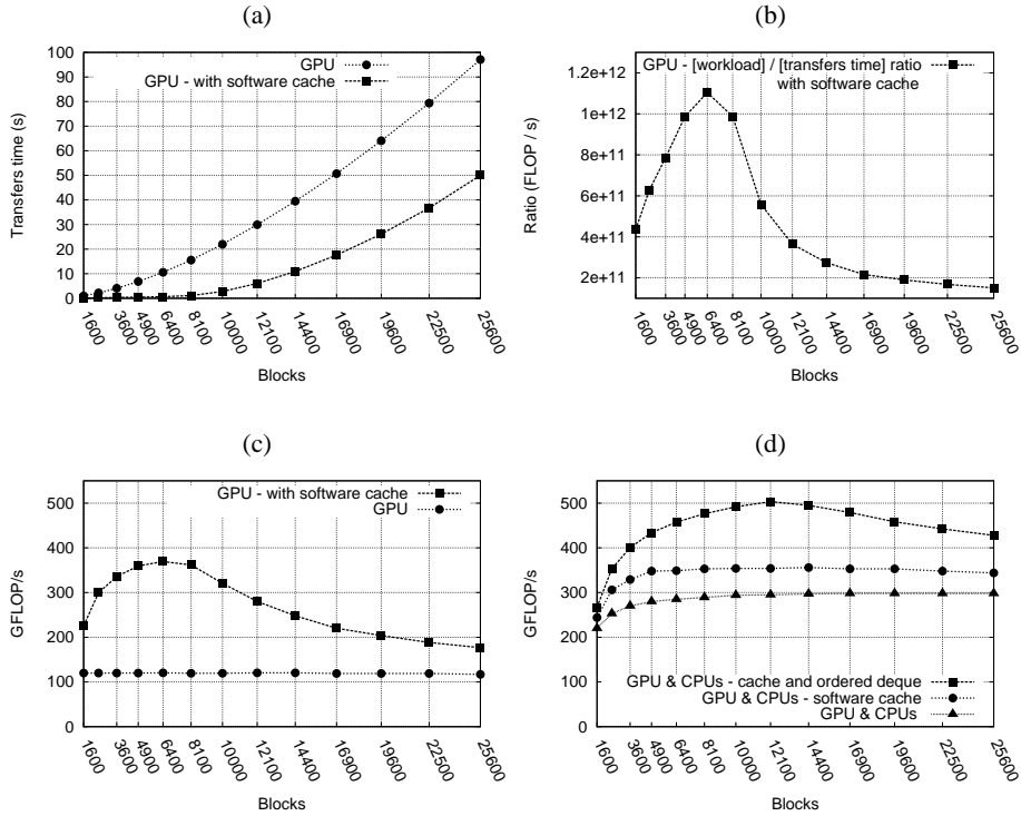
Fig. 6. Sparse LU step 3, single precision, average on 10 executions for each result: (a) cumulative time of all data transfers (b) ratio of workload to cumulative time of all transfers (c) GPU performance with and without software cache (d) heterogeneous execution and impact of the scheduler/cache interactions.
