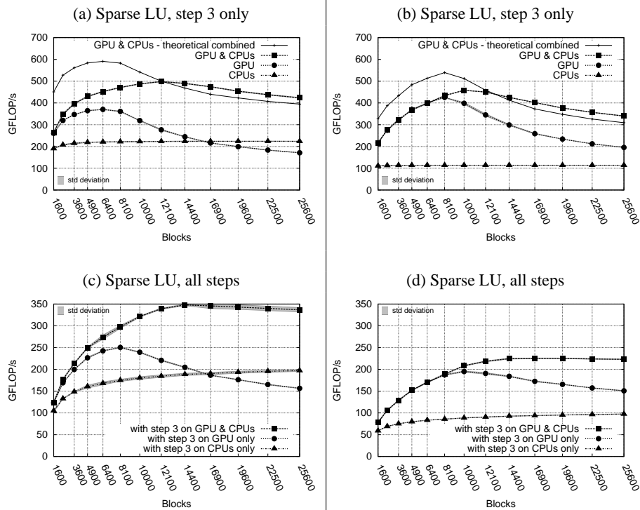
Fig. 7. Average on 25 executions for each result in single precision (the largest relative standard deviation is 2.25%): (a)(b) Step 3 only (c)(d) Global performance (step 3: GPU+CPUs, step 1&2: CPUs only).
