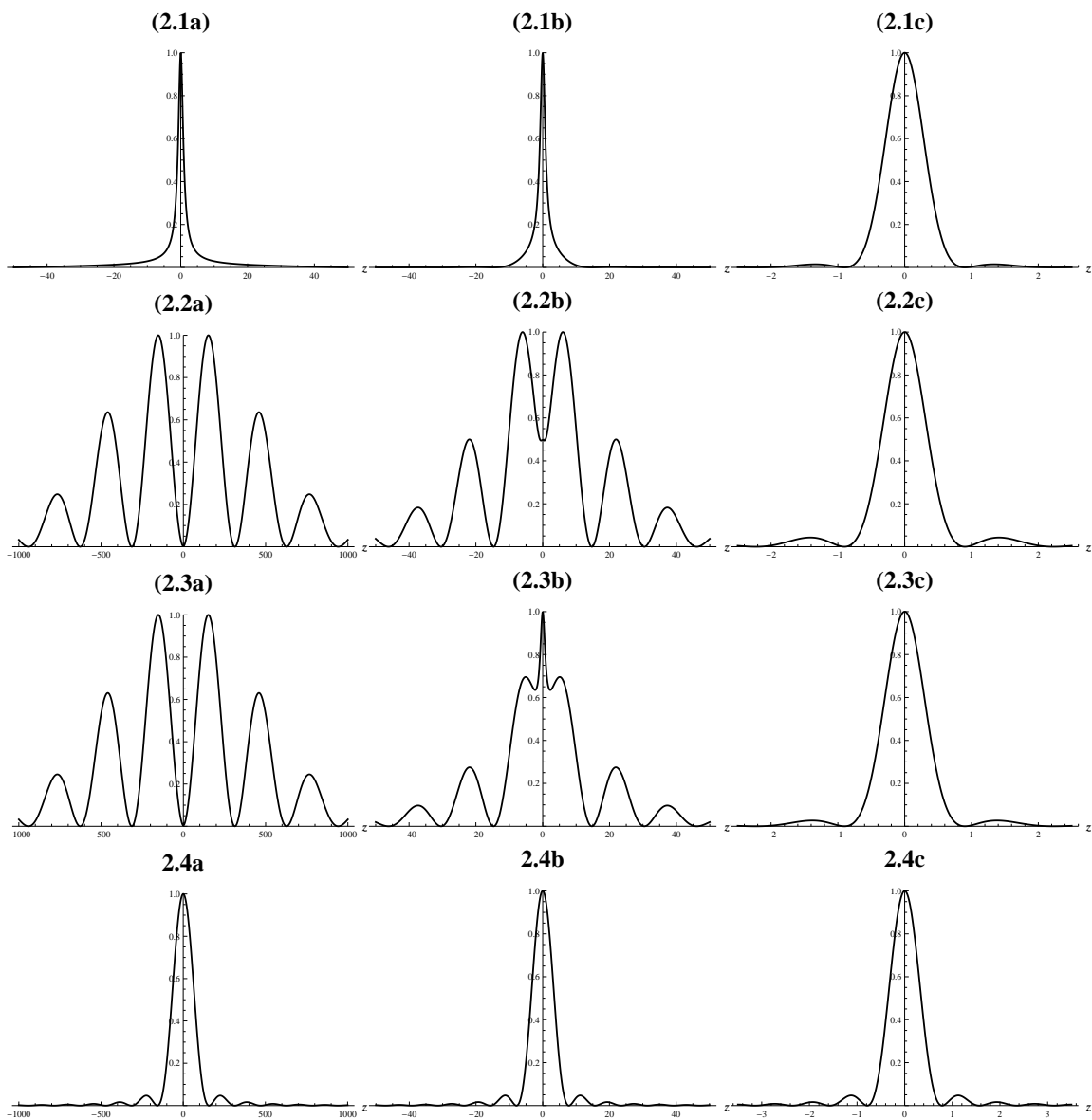
Figure 2: Semi-classical transition for the single-slit interference pattern. We take x = 1 , x_1 = 0 , x_0 = -1 , a = 0.01 and b = 0.1 in the units \hbar = m = 1 . We represent the relative populations computed as the square modulus of the propagators (28) respectively for the Dirichlet (Fig.2.1a-2.1c), Neumann (Fig.2.2a-2.2c) and free (Fig.2.3a-2.3c) boundary conditions and also for the truncation approximation (Fig.2.4a-2.4c) by the Equation (93), with t = 1 for the figures at the left (a), t = 0.05 at the middle (b) and t = 0.005 at the right (c).
