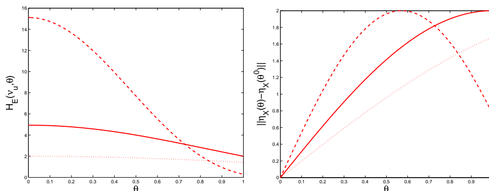
Figure 2: H_E(\nu_u, \theta) (left) and \|\eta_X(\theta) - \eta_X(\theta^0)\| (right) as functions of \theta \in \Theta = [0, 1] for r = 1 , u = 2 ( dotted line ), u = u_{\max} = 7\pi/4 ( dashed line ) and u = u_* = \pi ( solid line ).
