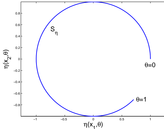
Figure 1: Expectation surface \mathbb{S}_\eta for \theta \in \Theta = [0, 1] , r = 1 and u = u_{\max} = 7\pi/4 .
