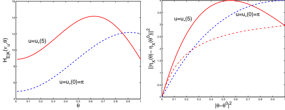
Figure 3: Left: H_{E|K}(\nu_u, \theta) as a function of \theta \in \Theta = [0, 1] ; right: \|\eta_X(\theta) - \eta_X(\theta^0)\|^2 and 2\phi_{eE|5}(\nu_{u_*(5)})|\theta - \theta^0|^2/(1 + K|\theta - \theta^0|^2) ( dash-dotted line ) as functions of |\theta - \theta^0|^2 ; u = u_*(5) ( solid line ) and u = u_*(0) = \pi ( dashed line ); r = 1 and K = 5 .
