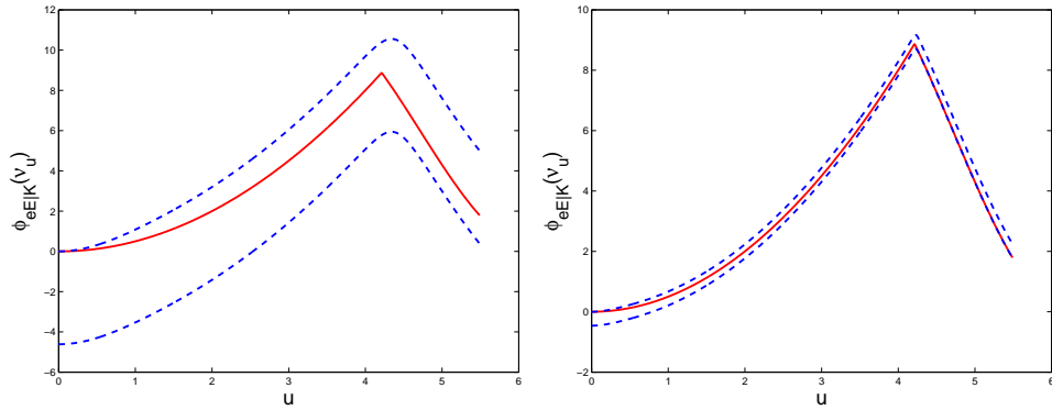
Figure 4: \phi_{eE}(\nu_u) ( solid line ) and upper and lower bounds (15) ( dashed lines ) as functions of u for \lambda = 1 (left) and \lambda = 10 (right).
