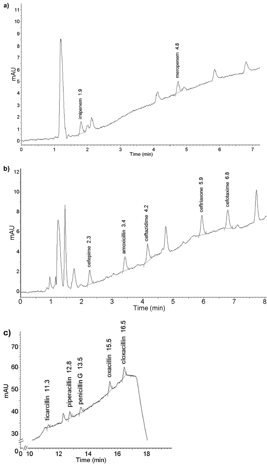
FIG. 1. HPLC chromatograms of an internal quality control with 10 \mu\text{g/ml} of each antibiotic at 298 nm (a), 230 nm (b), and 210 nm (c). Values after the antibiotic names are retention times.
