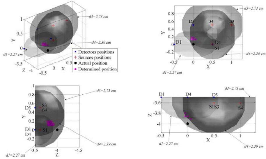
Fig. 4: Different points of view of the 3D surfaces for the measurement S1D1 ( d1=2.27\text{ cm} ), S3D3 ( d3=2.73\text{ cm} ) and S4D4 ( d4=2.39\text{ cm} ) merged with the actual position (plain dot marker) and the position of the fluorochrome defined by the intersection of the three 3D surfaces (star markers).
