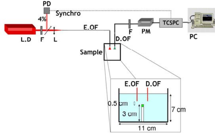
Fig. 1: Experimental time resolved setup. L.D.: Laser Diode; F: Filters; L: lens; PD: photodiode; E.OF: excitation optical fiber; D.OF: detection optical fiber; PM: photomultiplier; TCSPC: time correlated single photon counting system.
