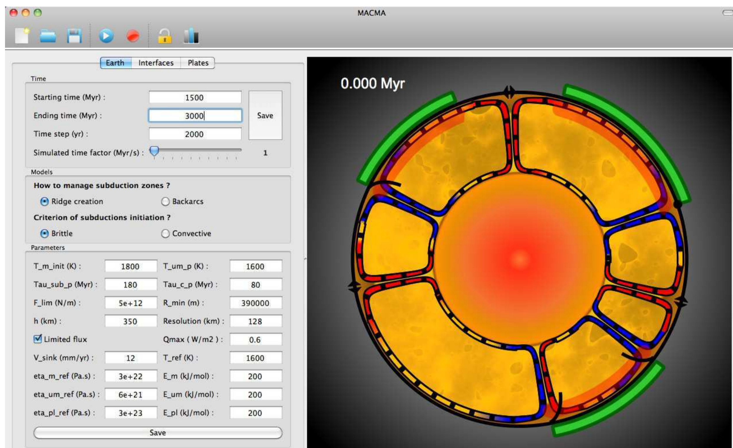
Fig. 1: Interface for MACMA: (left panel) geophysical input parameters and (right panel) evolutionary geometry of plates, convective cells, plate boundaries and continents.
