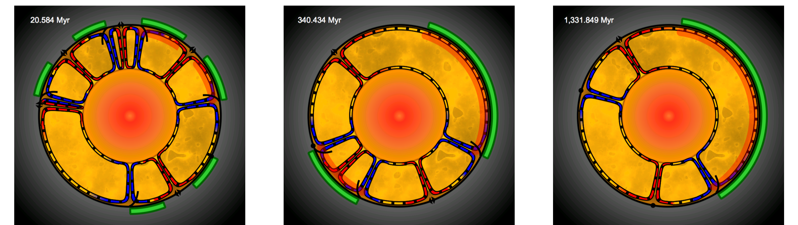
Fig. 4: Three configurations of plate tectonics obtained with the initial system shown in Fig. 1, showing the evolutive number of plates and continents.
