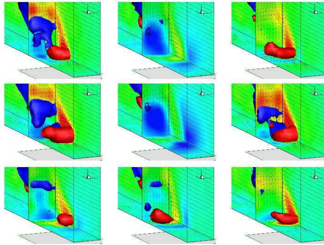
Figure 8: \omega_z iso-surfaces (red \omega_z > 0 – blue \omega_z < 0 , velocity vectors and velocity fluctuation iso-contours in 3 slices at 9 times separated by 0.8 s.
