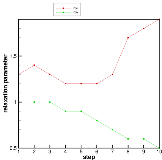
Figure 8: Best quality reconstruction relaxation parameter evolution with the number of MART steps. Figure 9: Comparison of ART and MART algorithms.
