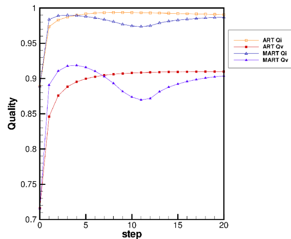
Figure 8: Best quality reconstruction relaxation parameter evolution with the number of MART steps. Figure 9: Comparison of ART and MART algorithms.
