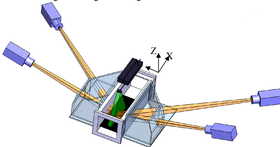
Figure 2: Cameras arrangement.
