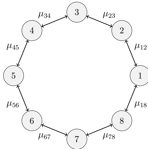
FIGURE 3. The graph relative to the Example 3.9 in the case n = 8 .
