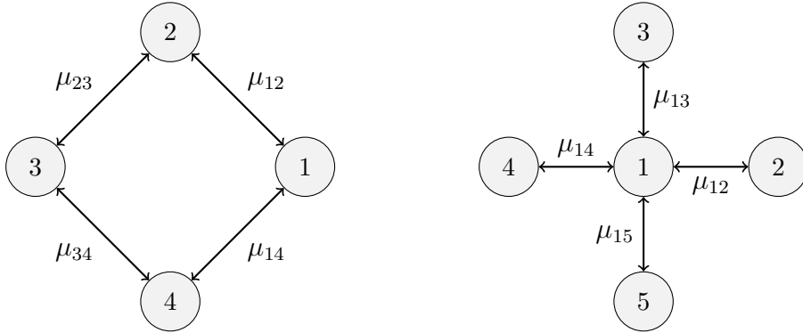
FIGURE 2. The graph relative to the Examples 3.4–3.5.
