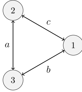
FIGURE 1. Schematic representation of the transitions in Examples 3.3.
