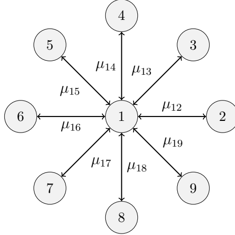
FIGURE 4. The graph relative to the Example 3.9 in the case n = 9 .
