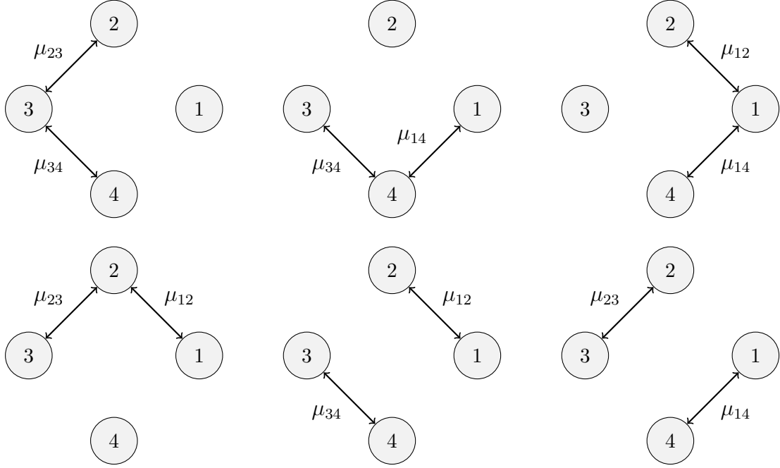
FIGURE 5. The six elements of \mathcal{F}_2 for the graph of the Example 3.4.
