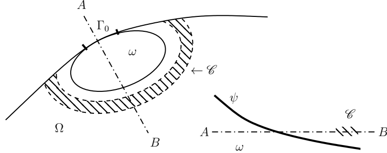
Figure 2: Construction of the weight function \psi(x) .
