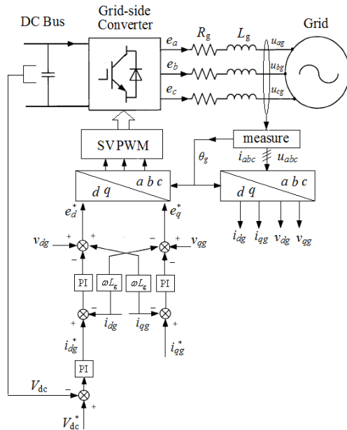
Figure 10. Control scheme of the grid-side converter.
