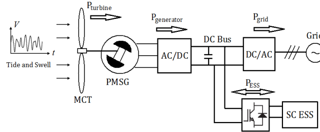
Figure 1. General scheme for a direct-drive MCT system with ESS.
