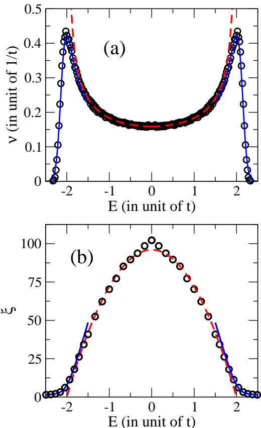
FIG. 3: (a) Density of states per site \nu as a function of energy E for the 1D Anderson model (12) with disorder amplitude W/t = 1 , in the limit N \rightarrow \infty . The circles correspond to numerical data (obtained with N = 1600 ). The red dashed line and the blue line are the theoretical predictions (17) and (18), expected in the bulk and at the edges of the manowire conduction band. (b) Localization length \xi of the 1D Anderson model (12) (with W/t = 1 ) as a function of energy E . The circles correspond to numerical data (obtained with Eq. (20)). The red dashed line and the blue line are the theoretical predictions (21) and (22).
