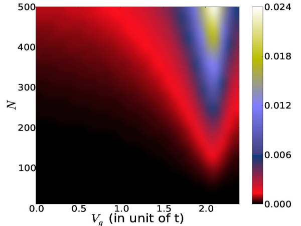
FIG. 8: (Color online) Typical value of the figure of merit ZT = \mathcal{S}^2/\mathcal{L}_0 = \pi^2/3(k_B T/t)^2 S^2 as a function of V_g and N , at E_F = 0 , W = t , and for a very low temperature k_B T/t = 5 \times 10^{-5} (which is nevertheless the highest temperature below which the Sommerfeld expansion is valid, for all N \leq 500 and V_g \leq 2.5t , within a tolerance of \sim 2\% , see Sec. VII). Being proportional to S^2 in the regime of validity of the Wiedemann-Franz law, the largest typical figures of merit are obtained around the edge of the impurity band and for long wires.
