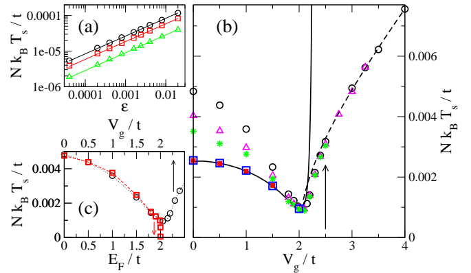
FIG. 9: (Color online) Temperature scale T_s above which the WF law breaks down. (a) Nk_B T_s/t as a function of the desired precision \epsilon on \mathcal{L} . The critical temperatures were extracted for different values of V_g ( V_g = t ( \circ ), 1.5t ( \square ), 2.02t ( \triangle )), with E_F = 0 , W/t = 1 , N = 500 and 1D leads. The solid lines are fits T_s = T_s^* \sqrt{\epsilon} . (b) Nk_B T_s/t (extracted for \epsilon = 4 \times 10^{-5} ) as a function of V_g/t , for chains of different length ( N = 150 ( \circ ), 300 ( \triangle ), 500 ( * ), 1500 ( \square ) and 3000 ( \blacksquare )), with E_F = 0 , W/t = 1 and 1D leads. The solid line is 4.04 \times 10^{-3} / (\nu_F t) , the dashed line is 4.37 \times 10^{-3} \sqrt{(V_g/2t)^2 - 1} and the arrow indicates the position of the edge of the impurity band. (c) Nk_B T_s/t (extracted for \epsilon = 4 \times 10^{-5} ) as a function of E_F/t at V_g = 0 ( \square ) and as a function V_g/t at E_F = 0 ( \circ ), with N = 150 , W/t = 1 and 1D leads. Dashed lines are guides to the eye.
