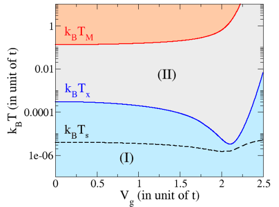
FIG. 1: (Color online) Typical temperature scales separating the different regimes of electronic transport (elastic regime ( T < T_x , blue), VRH regime ( T_x < T < T_M , gray) and activated regime ( T > T_M , red)) through a disordered nanowire. V_g is the external gate voltage which allows to lower the carrier density in the nanowire (it is completely depleted at V_g = 2.5t ). This paper is restricted to the study of region (I) at T < T_s where the Sommerfeld expansion can be applied for the calculation of the thermoelectric coefficients. Region (II) of VRH will be studied in Ref. 7 . The temperature scales T_s , T_x = \xi/(2\nu N^2) and T_M = 1/(\xi\nu) are plotted for the 1D model introduced in Sec. III with E_F = 0 , W = t and N = 1000 . T_s is given for \epsilon = 0.01\% (see Sec. VII).
