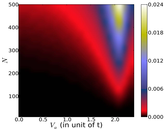
FIG. 8: (Color online) Typical value of the figure of merit ZT = S^2/\mathcal{L}_0 = \pi^2/3(k_B T/t)^2 S^2 as a function of V_g and N , at E_F = 0 , W = t , and k_B T/t = 5 \times 10^{-5} (the temperature was chosen as the highest temperature below which the Sommerfeld expansion is valid, for all N \leq 500 and V_g \leq 2.5t , within a tolerance of \sim 2\% , see Sec. VII). Being proportional to S^2 in the regime of validity of the Wiedemann-Franz law, the largest typical figures of merit are obtained around the spectrum edge and for long wires.
