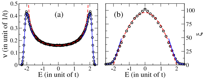
FIG. 3: (a) Density of states per site \nu as a function of energy E for the 1D Anderson model (12) with disorder amplitude W/t = 1 , in the limit N \rightarrow \infty . The circles correspond to numerical data (obtained with N = 1600 ). The red dashed line and the blue line are the theoretical predictions (16) and (17), expected in the bulk and at the edges of the manowire conduction band. (b) Localization length \xi of the 1D Anderson model (12) (with W/t = 1 ) as a function of energy E . The circles correspond to numerical data (obtained with Eq. (19)). The red dashed line and the blue line are the theoretical predictions (20) and (21).
