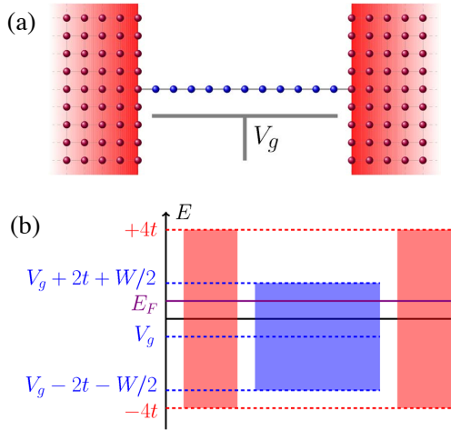
FIG. 2: (Color online) (a) Sketch of the system: a 1D nanowire made of N sites is connected to two leads at its extremities. An external gate voltage V_g is applied. (b) Band diagram. The energy spectrum of the nanowire (in blue) can be shifted by the application of V_g in order to probe either the bulk, the edges or the outside of the nanowire spectrum (conduction band of the nanowire when N \rightarrow \infty ) at Fermi energy E_F . Here, the leads are bidimensional (conduction band of the leads in red) and hence, E_F \in [-4t, 4t] .
