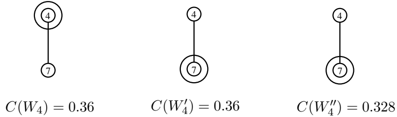
Figure 10: Substructures W_4 , W'_4 and W''_4 .
