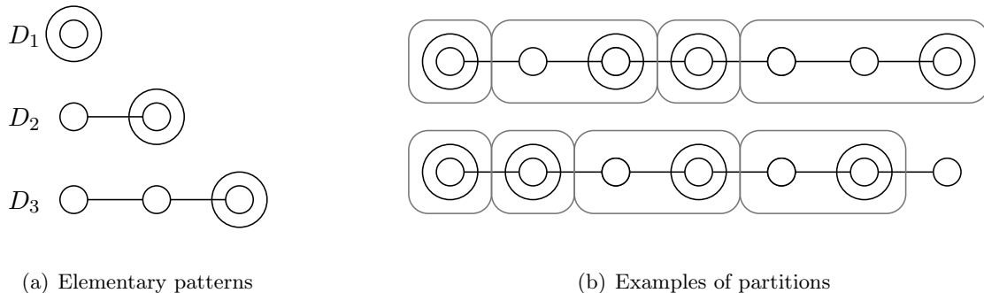
Figure 4: Partitioning nodes with elementary patterns.
