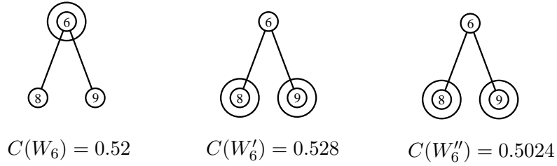
Figure 9: Substructures W_6 , W'_6 and W''_6 .
