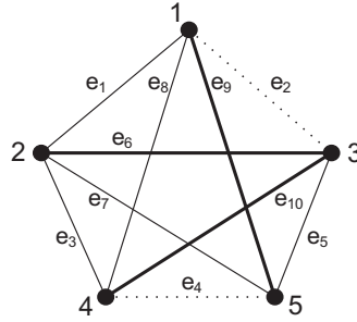
Figure 1: A fractional extreme point of the linear relaxation of the TNHNDP with L = 3 and \{s, t\} = \{1, 4\} .
