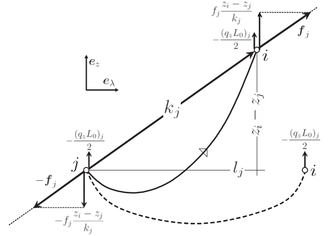
Fig. 4. Representation of the effective traction force f_j in the plane z - \lambda in the case of the truss, parabolic and catenary element.
