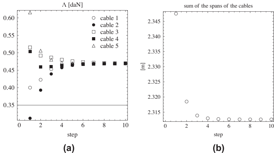
Fig. 11. URS strategy: (a) Convergence of the thrusts to the common value. (b) Minimization of the sum of the horizontal spans of the cables.
