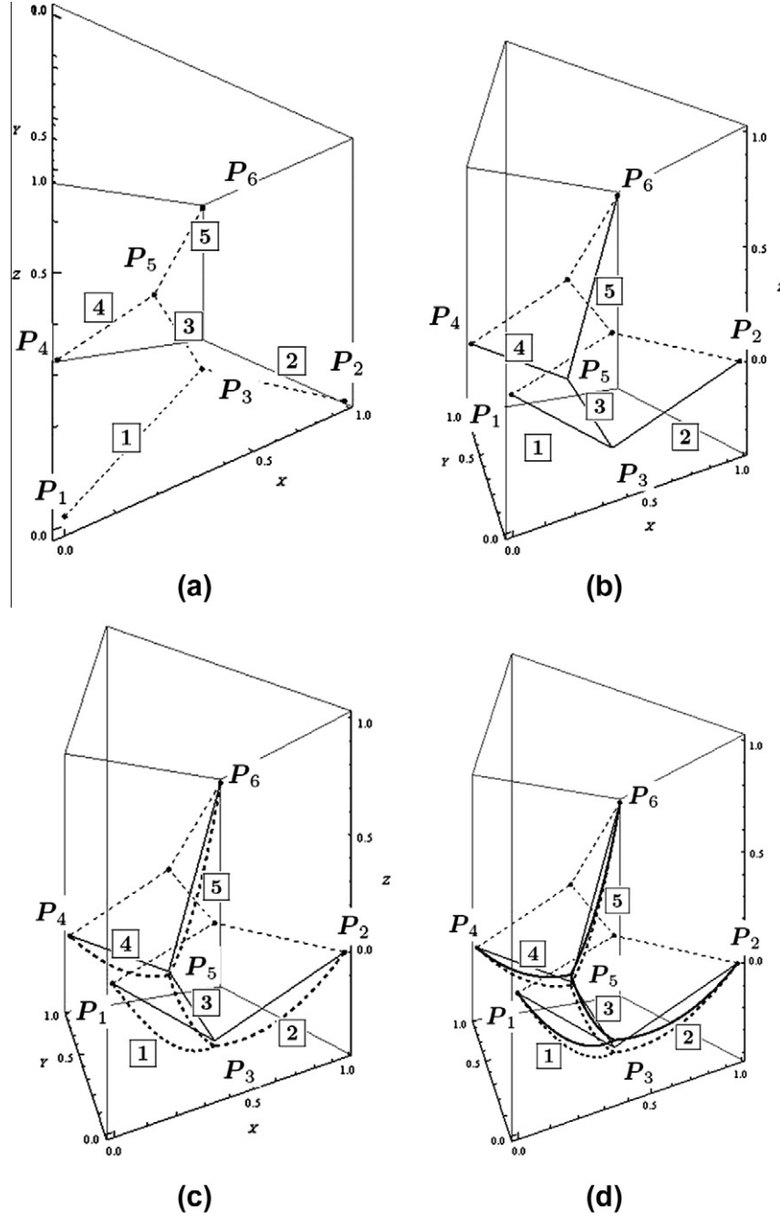
Fig. 7. Graphics representation of the configuration of a 5-cables net obtained for a self weight q_{z_j} = 1 [daN/m], j = 1, 2, n ; in (a) is plotted the solution of the linear force density method, (FDM), in (b) is plotted the solution of the non linear force density method, (nlFDM), in (c) is plotted the solution of the parabolic force density method, (P-FDM) and in (d) is plotted the solution of the catenary force density method, (C-FDM).
