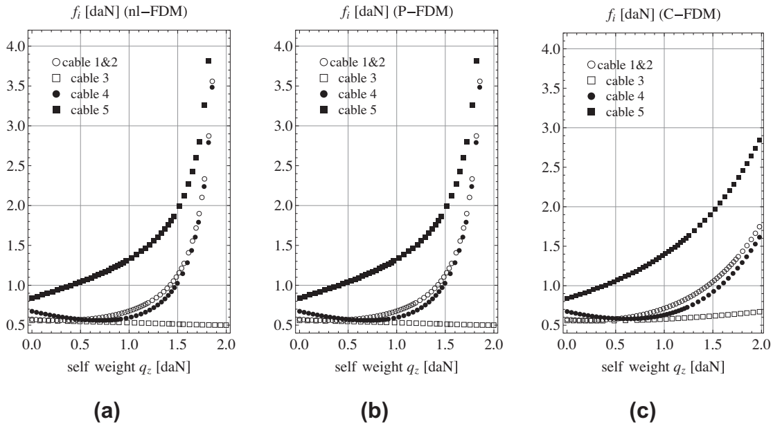
Fig. 6. Values of f_i for each cable, in the case of nl-FDM (a), P-FDM (b), and C-FDM (c). Q_A = 1 [daN/m], \eta = q_z / (2Q_A) , see Fig. 7.
