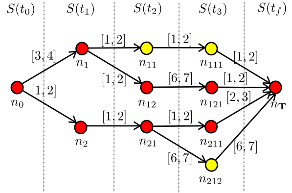
Figure 7: A graph example. Each node corresponds to a set of cells. The edges have interval weights corresponding to the costs J([\mathbf{u}_k]) of the control vectors [\mathbf{u}_k] \in \mathbf{U} . Note that n_0, n_1, n_2, n_{12}, n_{21}, n_{121}, n_{211} are reachable nodes whereas n_{11}, n_{111}, n_{212} are indeterminate nodes.
