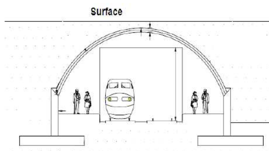
Figure 5 Protection tunnel
