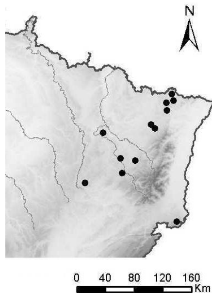
Figure 1. Location of sampled stands. Each dot corresponds to a stand-pair.
