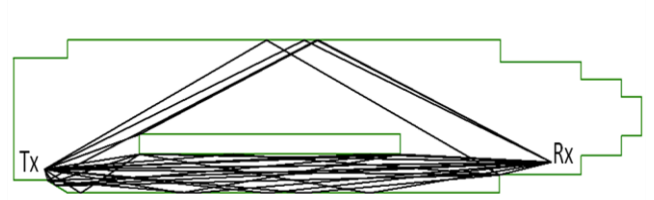
Figure 4. Ray-tracing results for the parking in LoS configuration.
