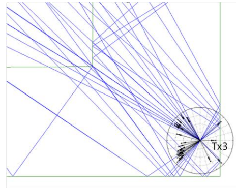
Figure 10. DoD results for the location Tx3.
