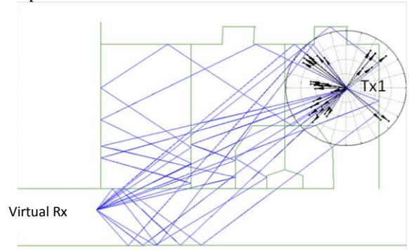
Figure 9. DoD results for the location Tx1.
