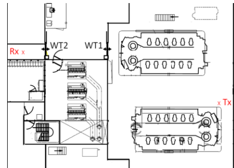
Figure 1. Tx and Rx locations in the engine rooms.
