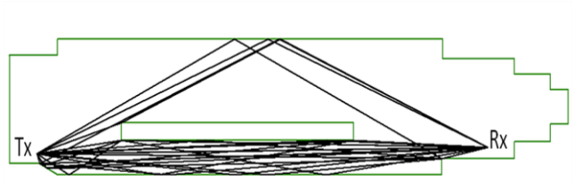
Figure 4. Ray-tracing results for the parking in LoS configuration.
