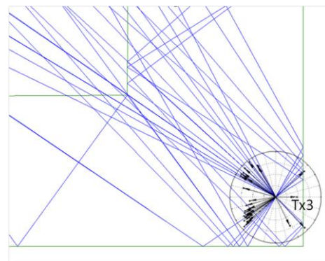
Figure 10. DoD results for the location Tx3.
