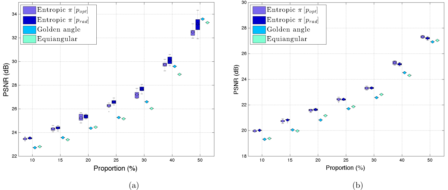
Figure 11: Box plots for PSNR of the reconstructed images with respect to the proportion of measurements chosen in the scheme (10%, 15%, 20%, 25%, 30%, 40%, 50%). Setting 512 \times 512 . (a) reconstruction for 'Barbara' as the reference image, (b) reconstruction for the 'Baboon' as the reference image.
