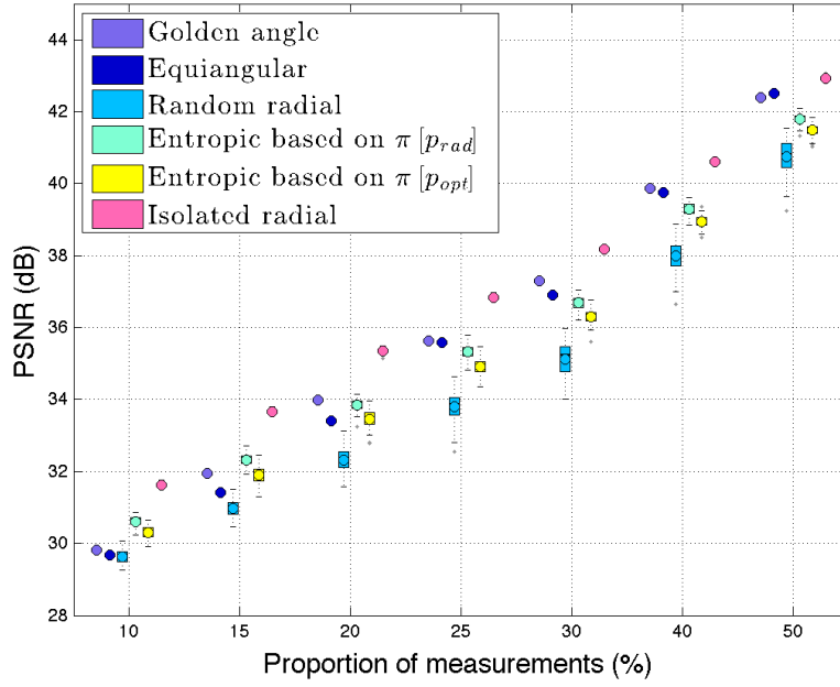
Figure 7: Box plots for PSNR of the reconstructed images with respect to the proportion of measurements chosen in the scheme (10%, 15%, 20%, 25%, 30%, 40%, 50%). Setting 256 \times 256 .
