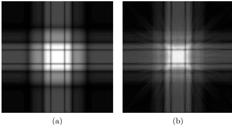
Figure 3: Illustration of the fidelity of \pi[\mathbf{p}_{\text{opt}}] to \mathbf{p}_{\text{opt}} . (a): on the left hand side, we present the target probability distribution \mathbf{p}_{\text{opt}} (b): on the right hand side, we perform 100000 i.i.d. drawings according to \pi[\mathbf{p}_{\text{opt}}] of blocks from the blocks dictionary and count the number of times that a point is sampled at each location.
