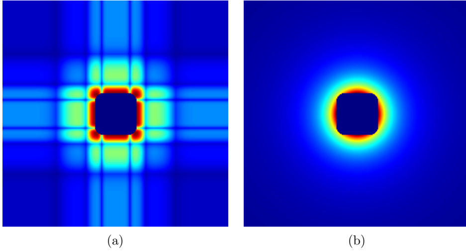
Figure 5: Target probabilities on pixels (in red, high values, and in dark blue, values near to 0). (a) displays the distribution proportional to \|\mathbf{a}_i^*\|_{\ell^\infty}^2 defined in [CCW13], (b) displays a radial distribution as presented in [KW12]. The center has been set to zero, since it will be sampled by the mask in a deterministic way.
