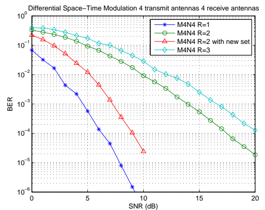
Fig. 4. Simulation results of the new differential space-time scheme for 4 transmit antennas and 4 receive antennas with spectral efficiency 1, 2 and 3 bps/Hz respectively.
